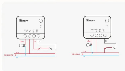
Wiring with 2-way Switch Control
