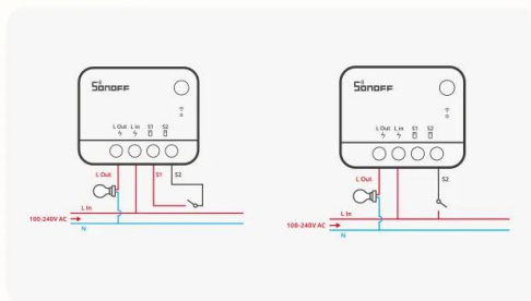
Wiring with One External Switch Control
