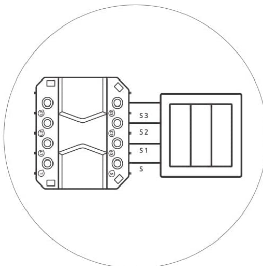
Connect S-MATE with your ordinary switch.
